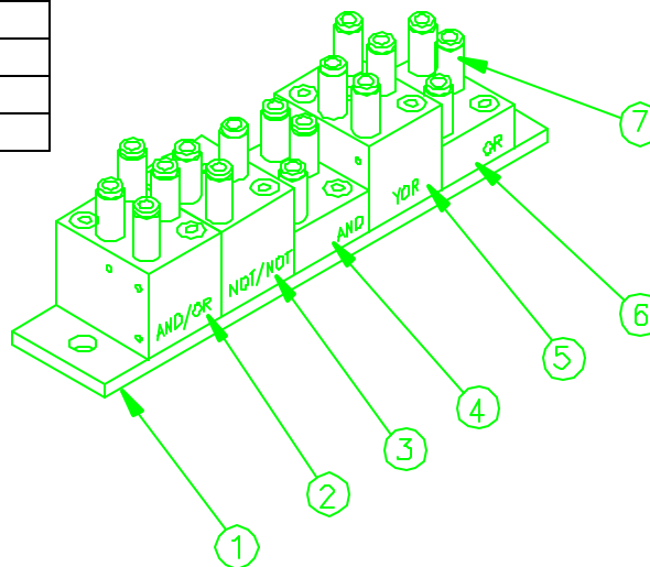
One-Hand Control Valve Pack (Part No. A-3321)
